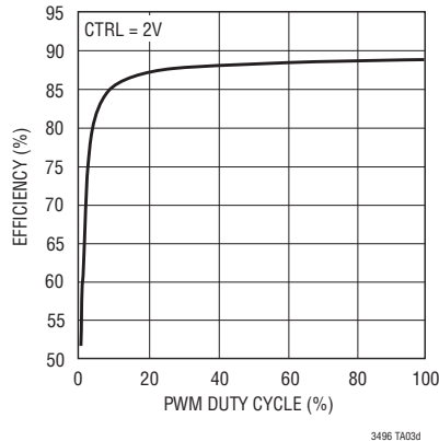
Efficiency vs PWM Duty Cycle
