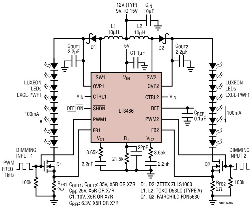
12V to 8/8 White LEDs
