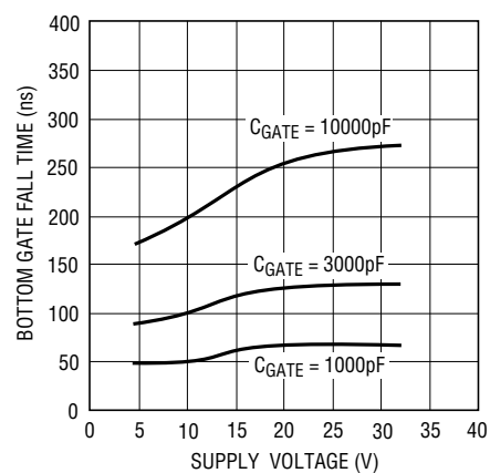
Bottom Gate Fall Time
