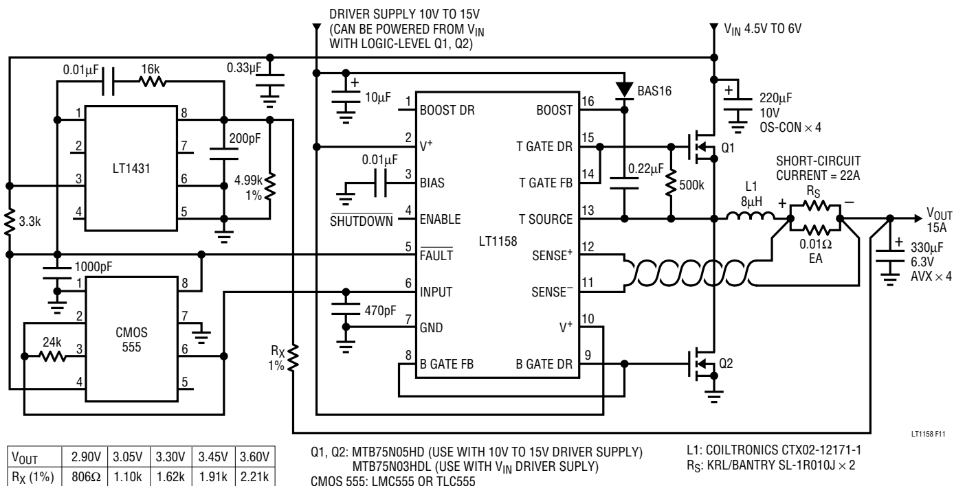
Figure 11. 5V to 3.XXV, 15A Converter (Uses PC Board Area for Heatsink)
