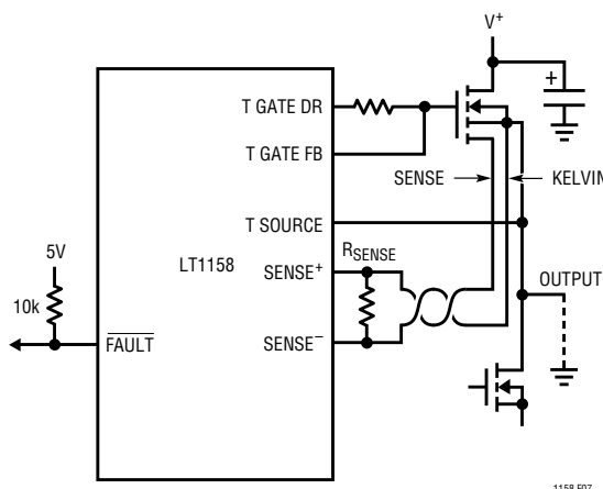
Figure 7. Short-Circuit Protection with Current-Sensing MOSFET
