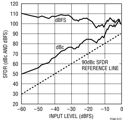
LTC2246: SFDR vs Input Level, f_{IN} = 5\text{MHz} , 2V Range, 25Mpsps
