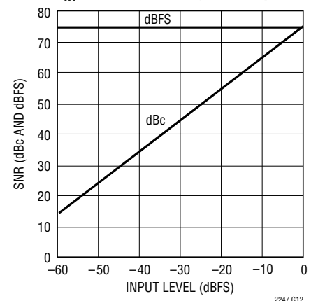
LTC2247: SNR vs Input Level, f_{IN} = 5\text{MHz} , 2V Range, 40Mps
