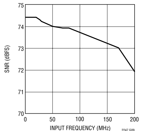
LTC2247: SNR vs Input Frequency, -1\text{dB} , 2V Range, 40Mps
