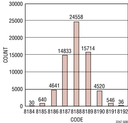
LTC2247: Grounded Input Histogram, 40Mps
