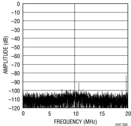
LTC2247: 8192 Point FFT, f_{IN} = 70\text{MHz} , -1\text{dB} , 2V Range, 40Mps
