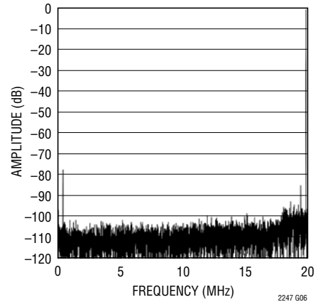
LTC2247: 8192 Point FFT, f_{IN} = 140\text{MHz} , -1\text{dB} , 2V Range, 40Mps
