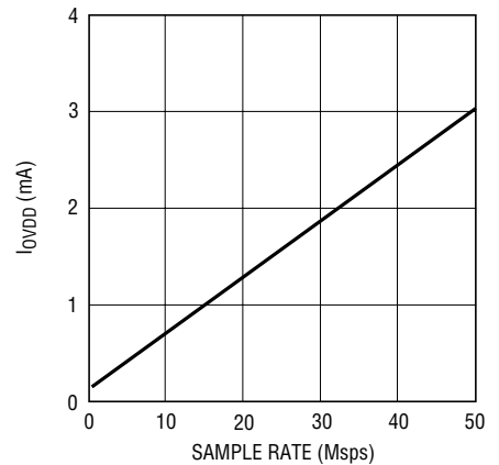
LTC2247: I_{VDD} vs Sample Rate, 5MHz Sine Wave Input, -1dB, O_{VDD} = 1.8\text{V}
