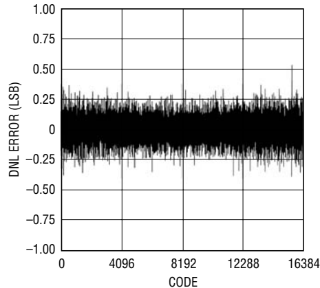
LTC2246: Typical DNL, 2V Range, 25Msps
