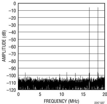
LTC2247: 8192 Point 2-Tone FFT, f_{IN} = 21.6\text{MHz} and 23.6\text{MHz} , -1\text{dB} , 2V Range, 40Mps
