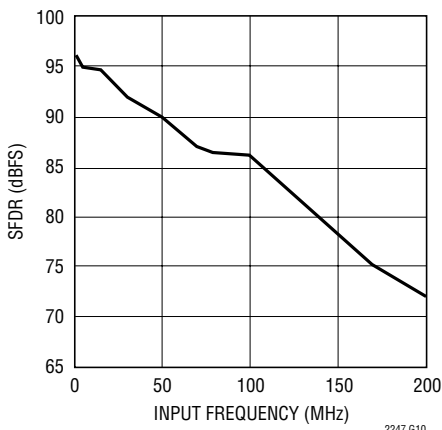
LTC2247: SFDR vs Input Frequency, -1\text{dB} , 2V Range, 40Mps
