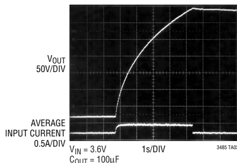
LT3485-0 Charging Waveform
