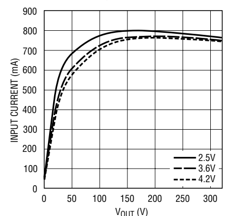
LT3485-3 Input Current
