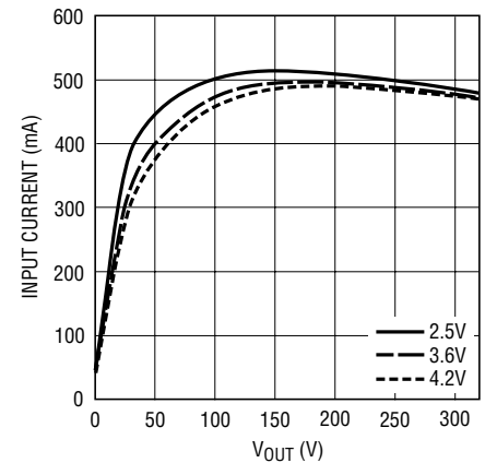
LT3485-0 Input Current
