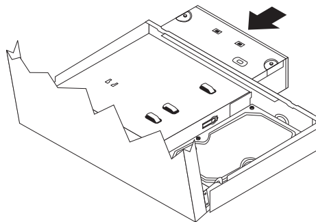
Figure 13. Installing the optical drive
