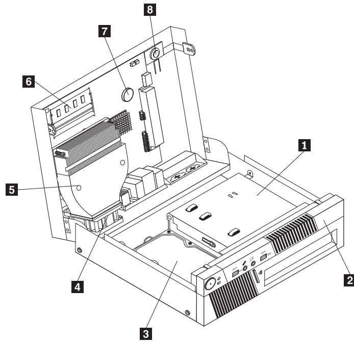
Figure 3. Component locations
