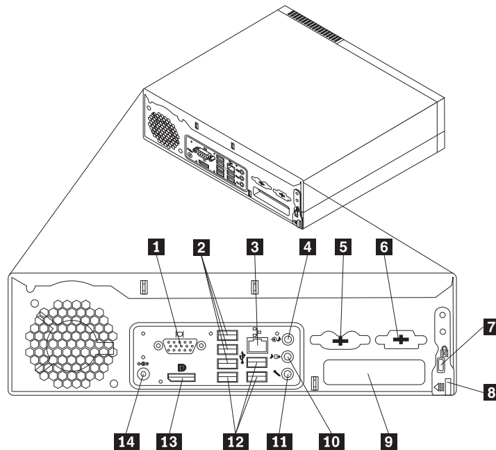
Figure 2. Rear connector locations
