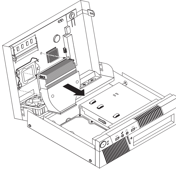
Figure 16. Removing the heat sink
