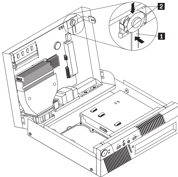
Figure 17. Removing the internal speaker
