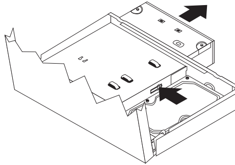
Figure 11. Removing the optical drive
