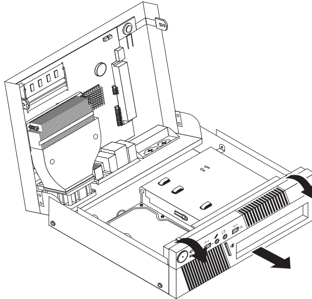
Figure 6. Removing the front bezel
