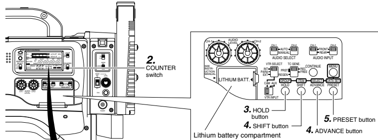
Time display (COUNTER switch: TC)
