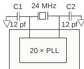
Figure 3-1. Crystal Configuration
