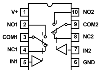
ISL84762 (TDFN, MSOP) TOP VIEW
