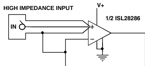
FIGURE 44. GUARD RING EXAMPLE FOR UNITY GAIN AMPLIFIER
