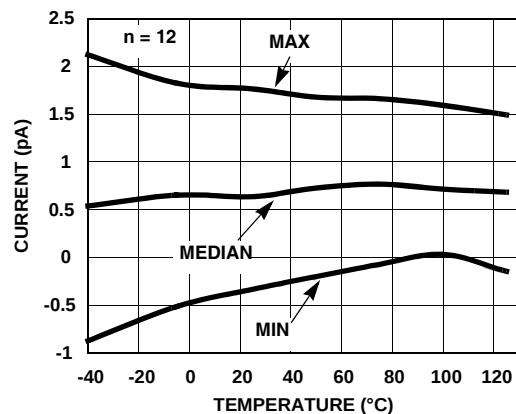
FIGURE 24. INPUT OFFSET CURRENT vs TEMPERATURE V_S = \pm 1.2V
