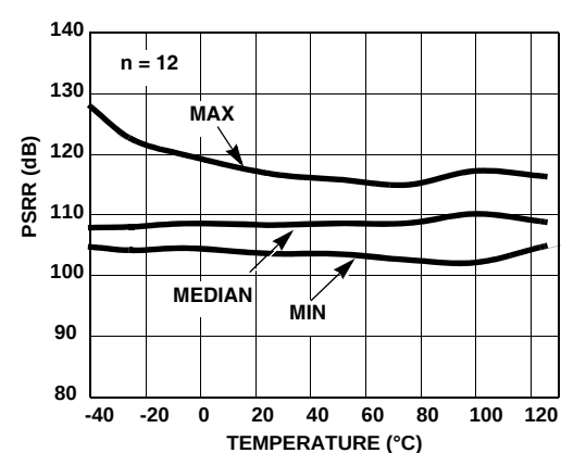
FIGURE 28. PSRR vs TEMPERATURE V_S = \pm 2.5V
