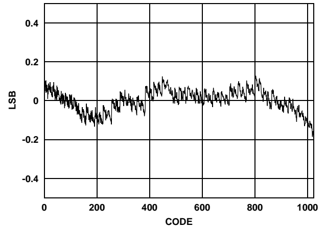
FIGURE 37. INTEGRAL NONLINEARITY
