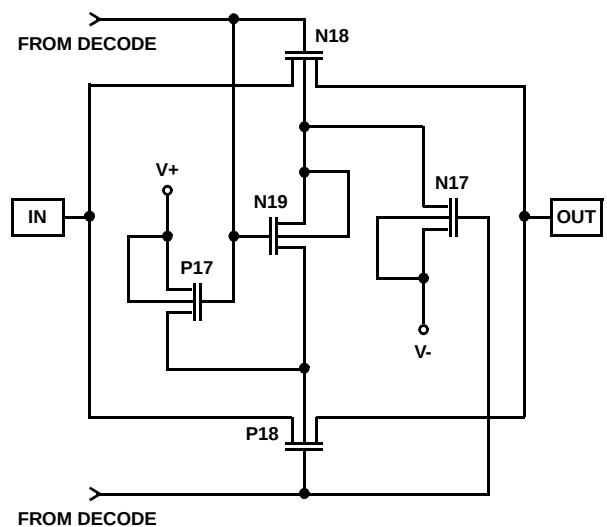
MULTIPLEX SWITCH
