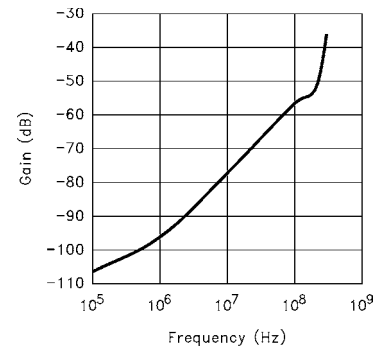
FIGURE 18. CHANNEL-CHANNEL ISOLATION
