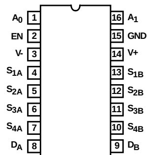
DG509A (PDIP, SOIC) TOP VIEW
