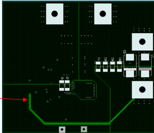
Fig. 26b. IRDC3843W demoboard layout considerations – Bottom Layer
