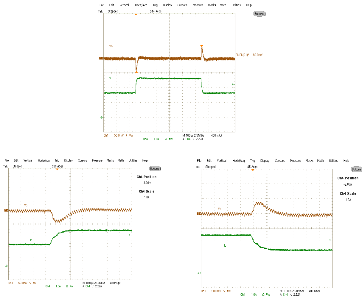
Fig. 23. Transient Response, 1A to 2A step 2.5A/μs Ch 1 :V o , Ch 4 :I o
