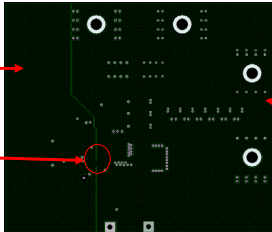
Fig. 26c. IRDC3843W demoboard layout considerations – Mid Layer 1
