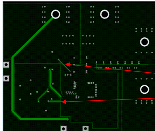
Fig. 26d. IRDC3843W demoboard layout considerations – Mid Layer 2
