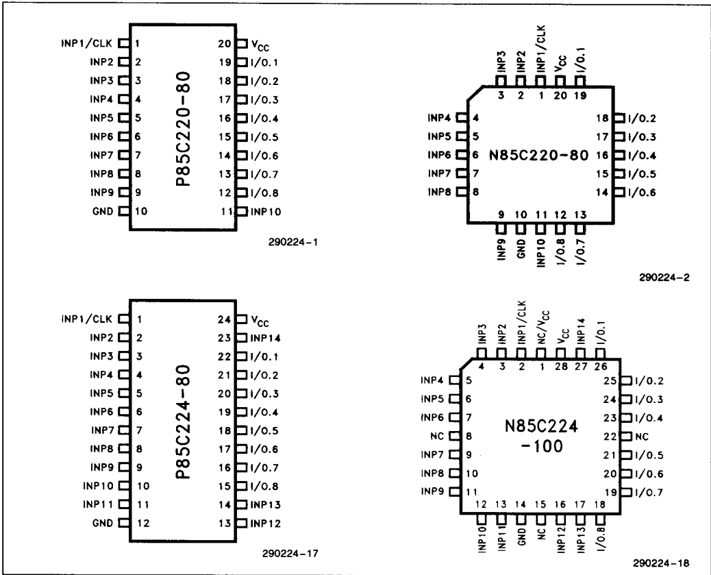
Figure 1. Pinout Diagrams
