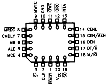
Figure 2. 82C288 Pin Configuration
