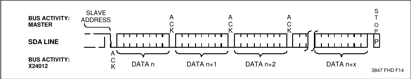
Figure 9. Sequential Read
