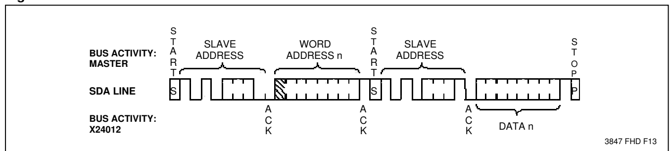
Figure 8. Random Read
