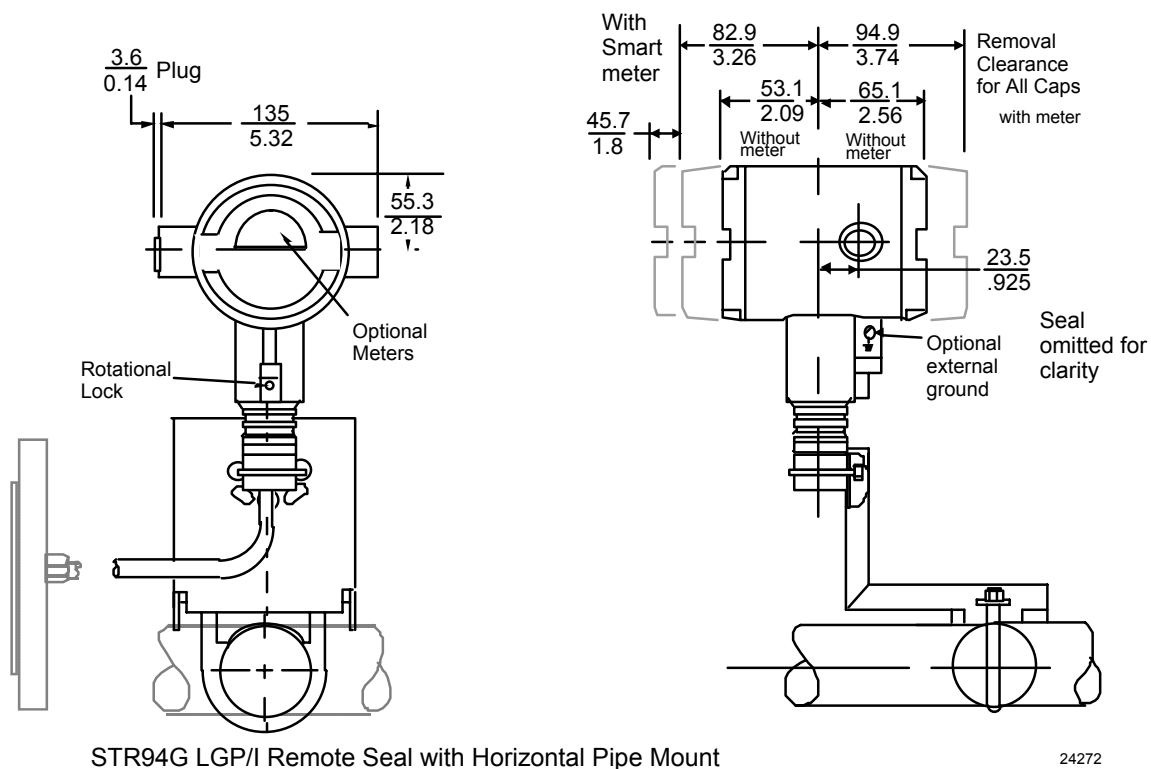
Figure 7 —Approximate horizontal mounting dimensions for Remote Seal Transmitter.
