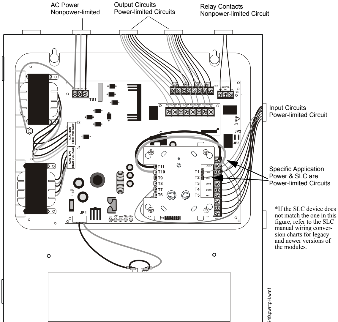
Figure 2.5 Power-limited Wiring Example
