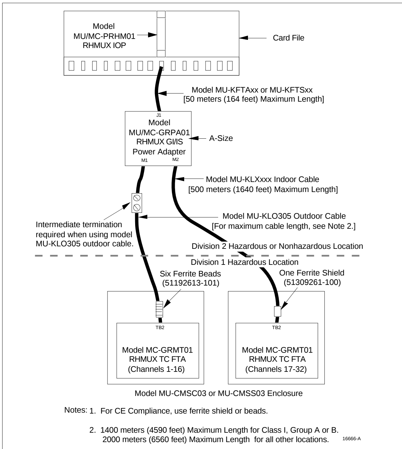
Figure 12-4 Intrinsically Safe RHMUX Configuration Interconnections
