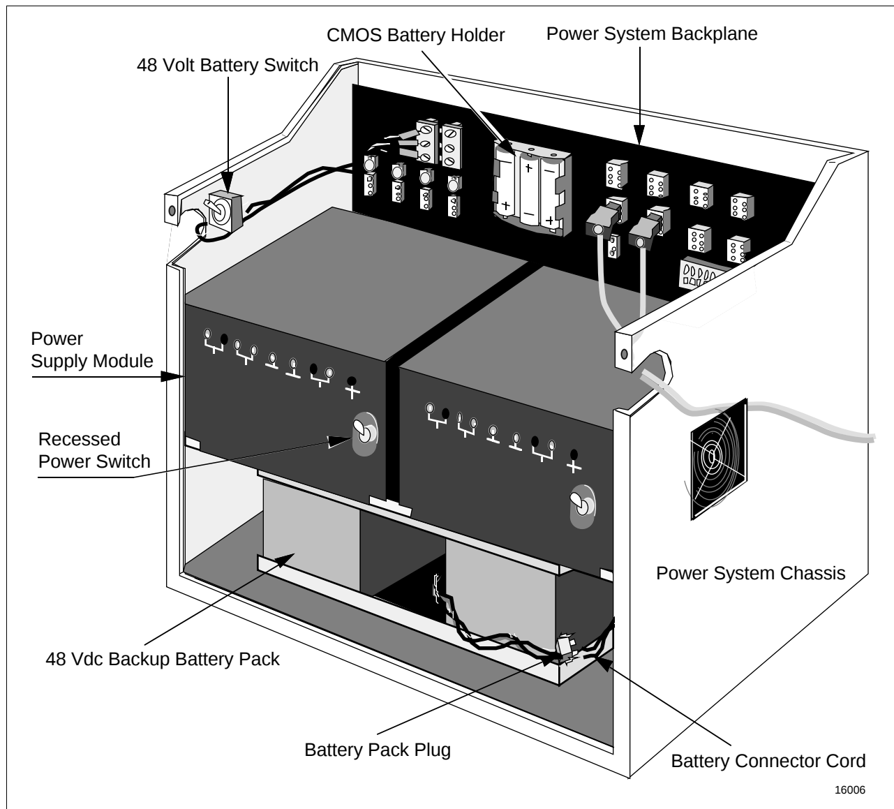
Figure 2-22 Standard Power System—Model MU-PSRX03
