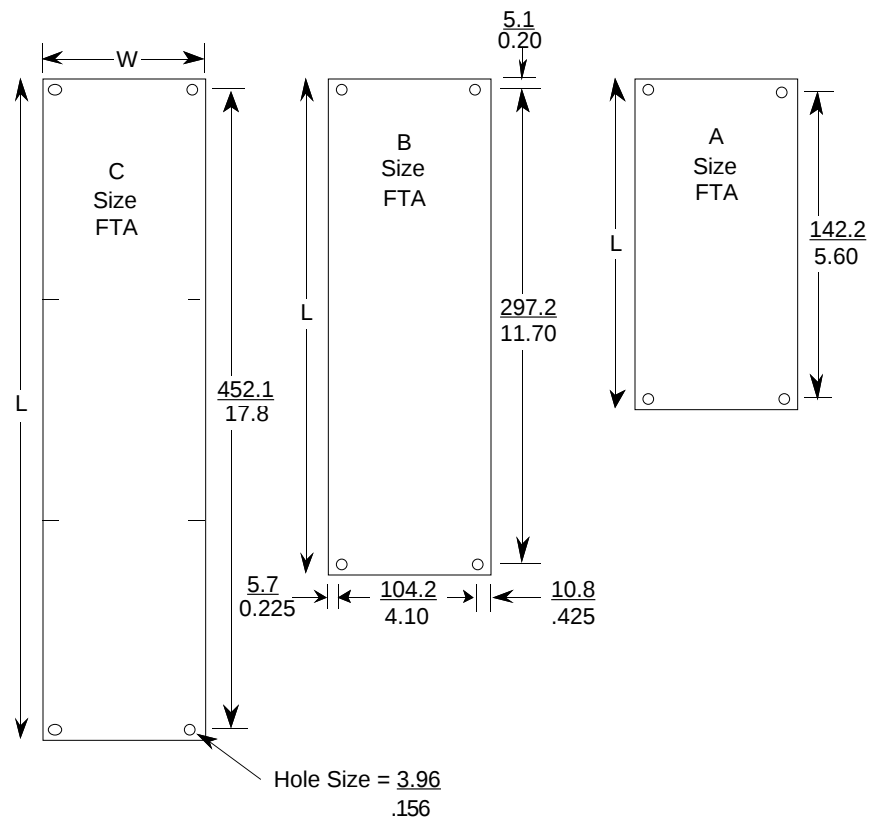
Figure 4-2 Field Termination Assembly (FTA) Mounting Dimensions
