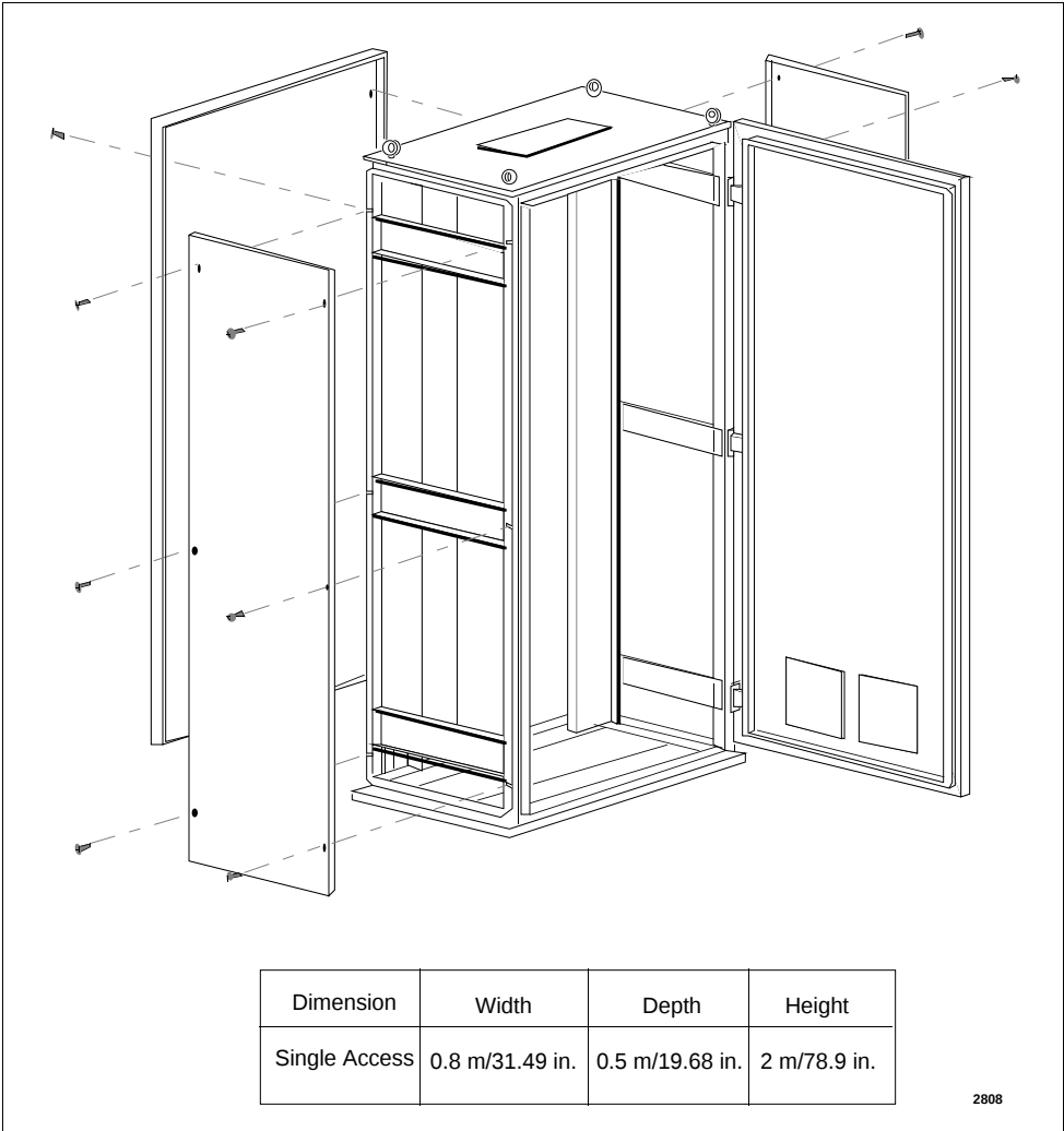
Figure 9-1 Single-Access Cabinet
