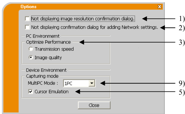
Fig. 4.c Option menu of Projector Models Group: B
