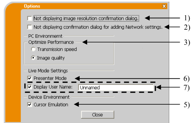
Fig. 4.d Option menu of Projector Models Group: C
