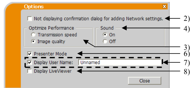
Fig. 4.f Option menu of Projector Models Group: E
