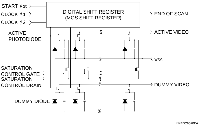
Figure 1 Equivalent circuit
