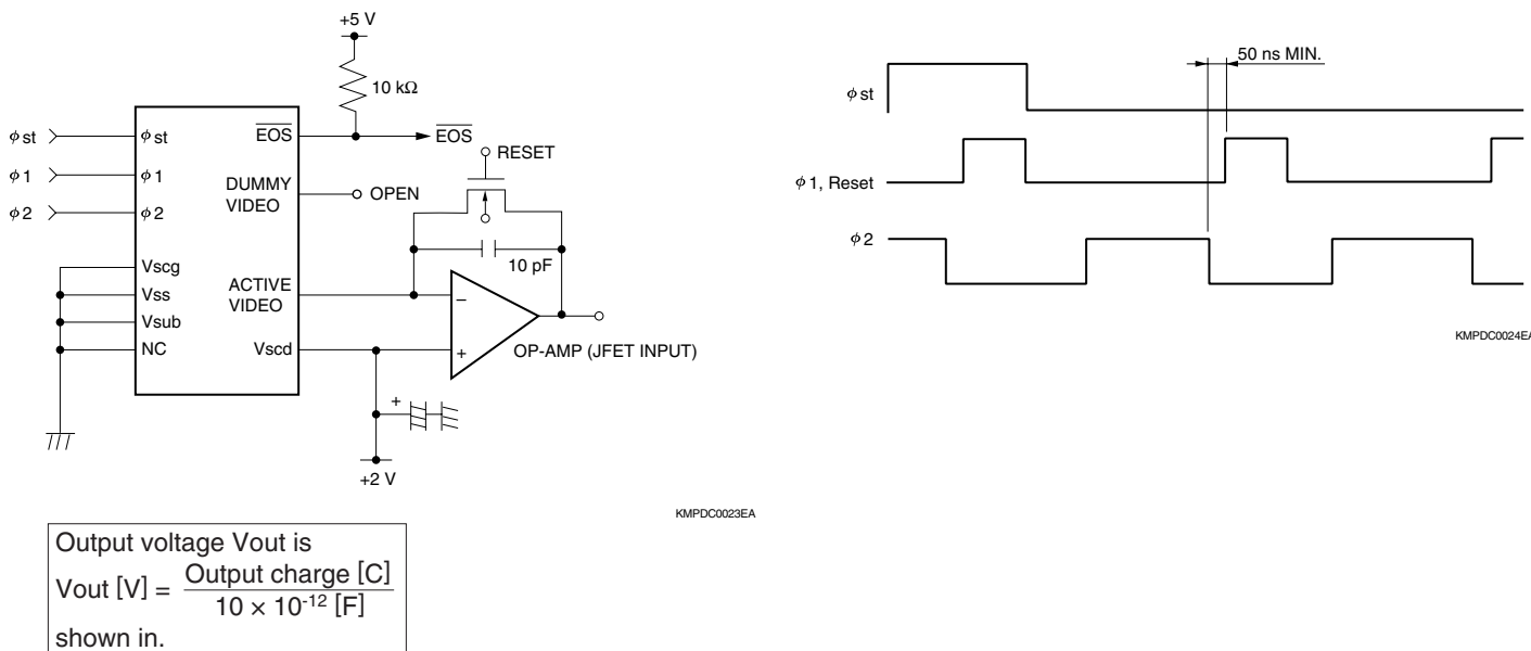
Figure 9 Readout circuit example and timing chart
