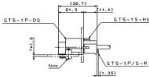
◆ Diagram of Mated Connector in Use
