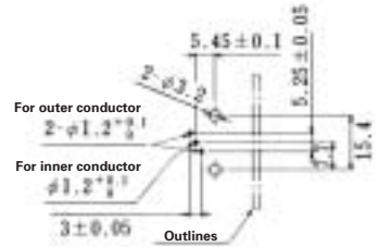
◆ Recommended PCB Mounting Pattern
