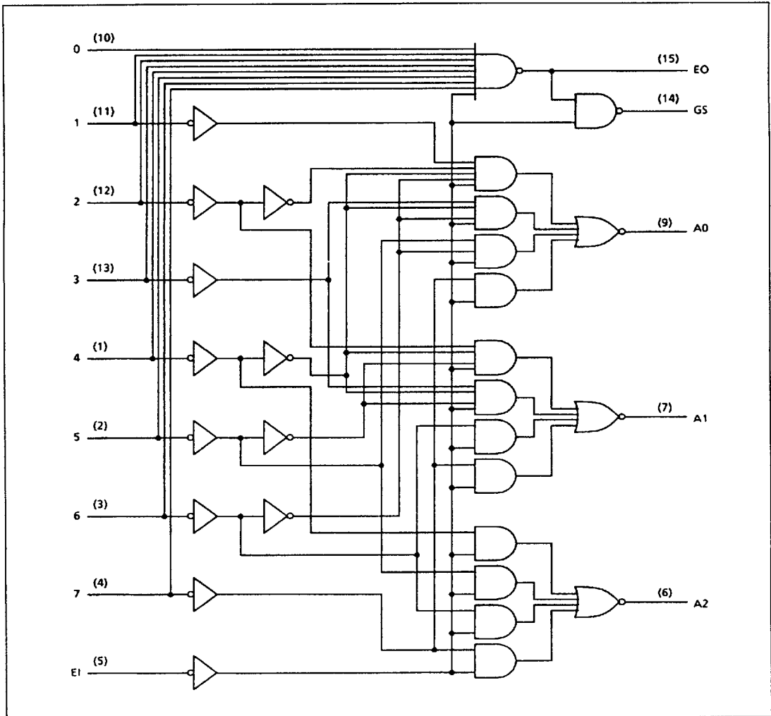
Figure 5: Logic Diagram
