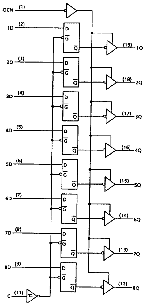
Figure 5: Logic Diagram
