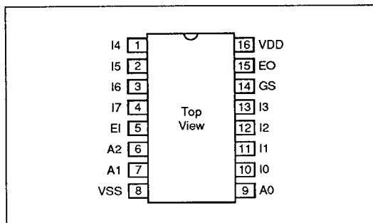
Figure 1: Pin Out
