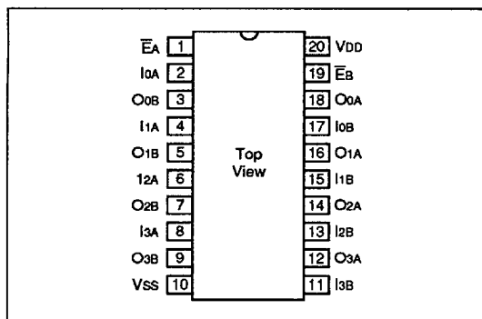
Figure 2: Pin Out
