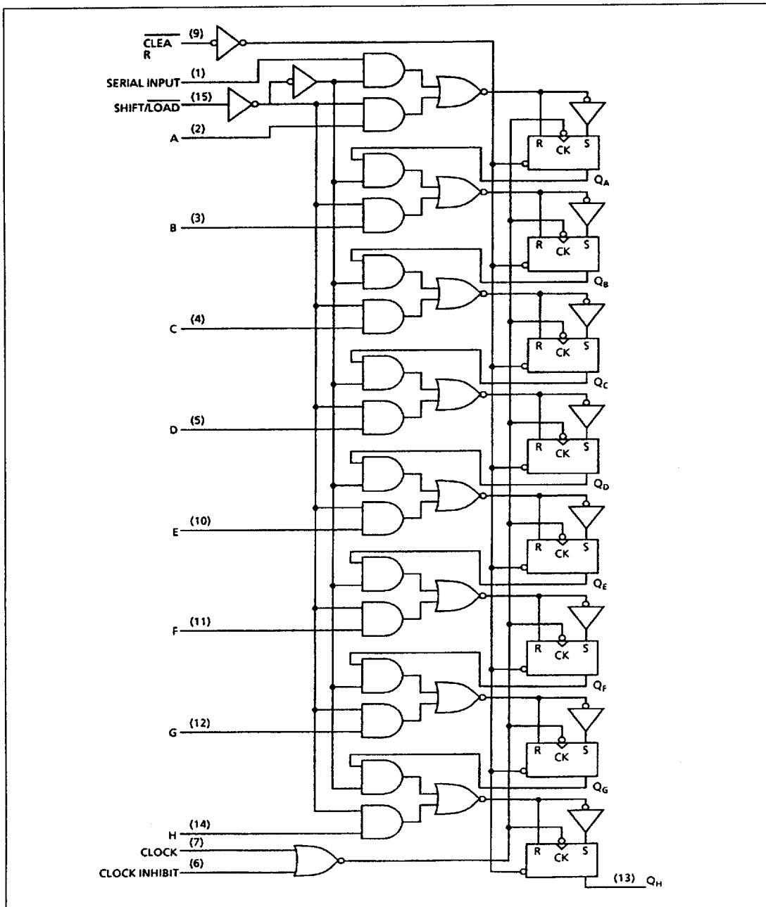
Figure 5: Logic Diagram
