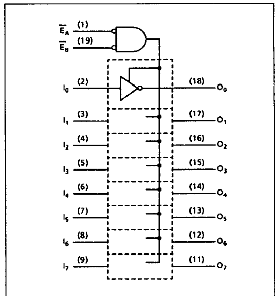
Figure 3: Logic Diagram
