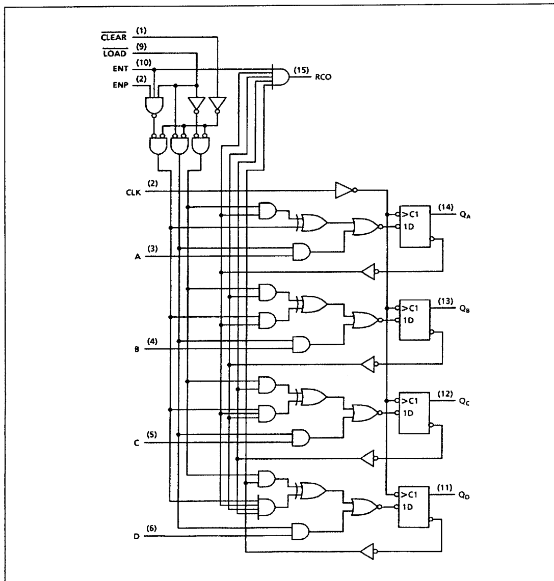
Figure 5: Logic Diagram
