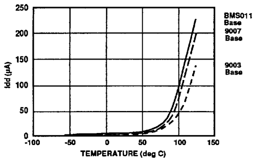
STATIC I_{dd} Vs TEMP.
