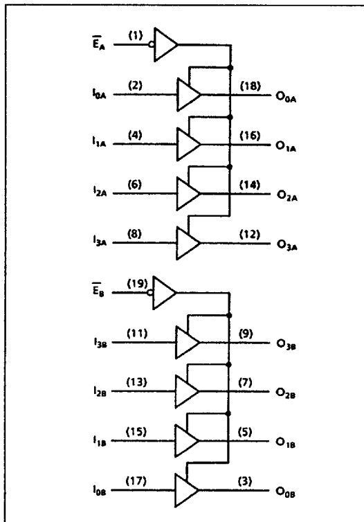
Figure 3: Logic Diagram
