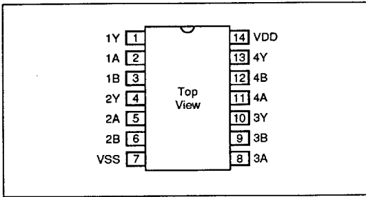
Figure 3: Pin Out
