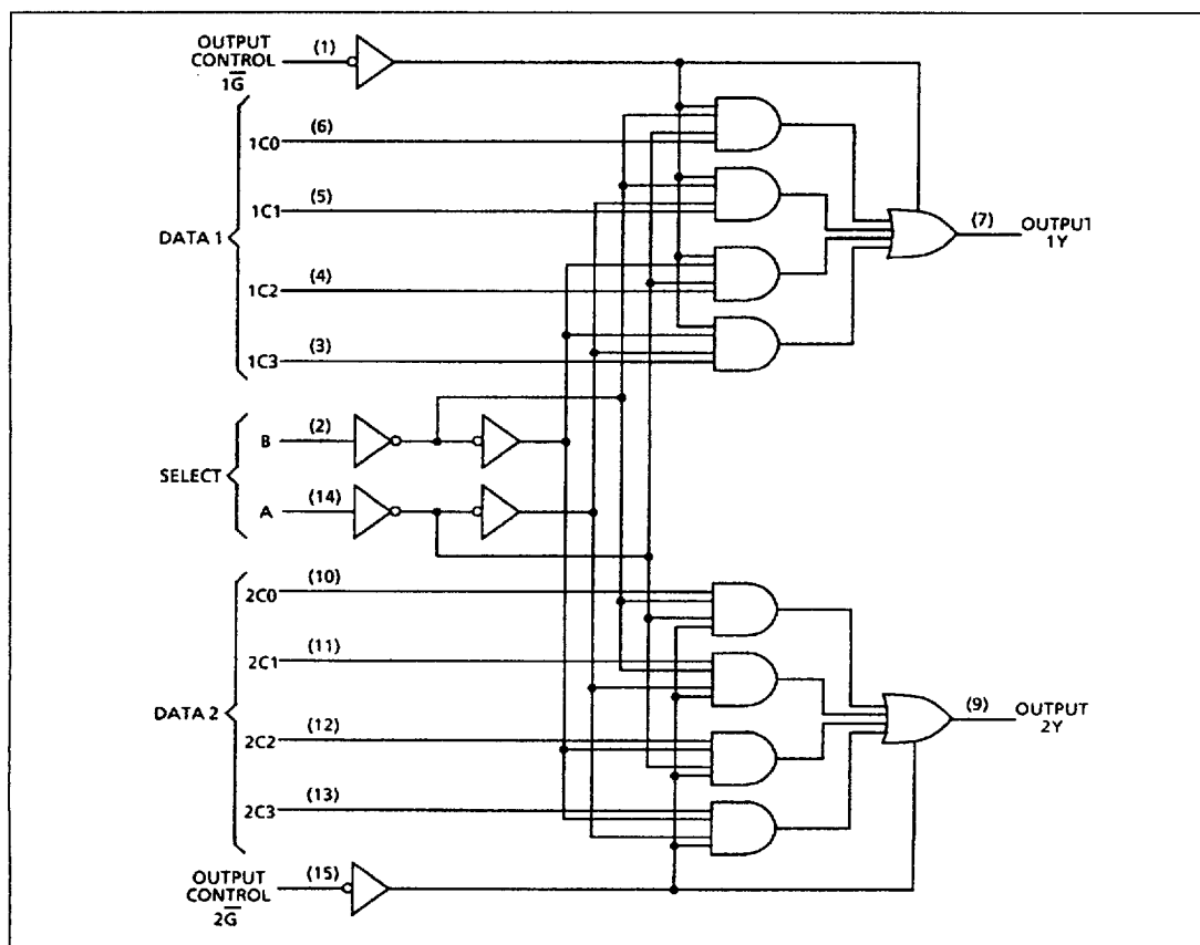
Figure 5: Logic Diagram
