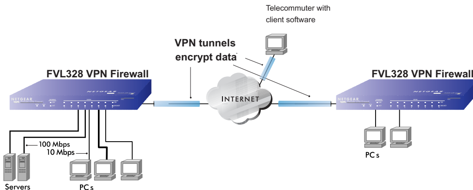
Figure 6-1: Secure access through FVL328 VPN routers
