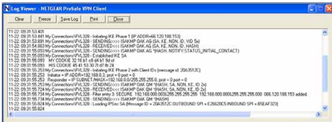
Figure H-14: Log Viewer screen
