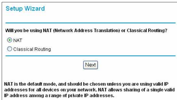
Figure 3-6: Setup Wizard
