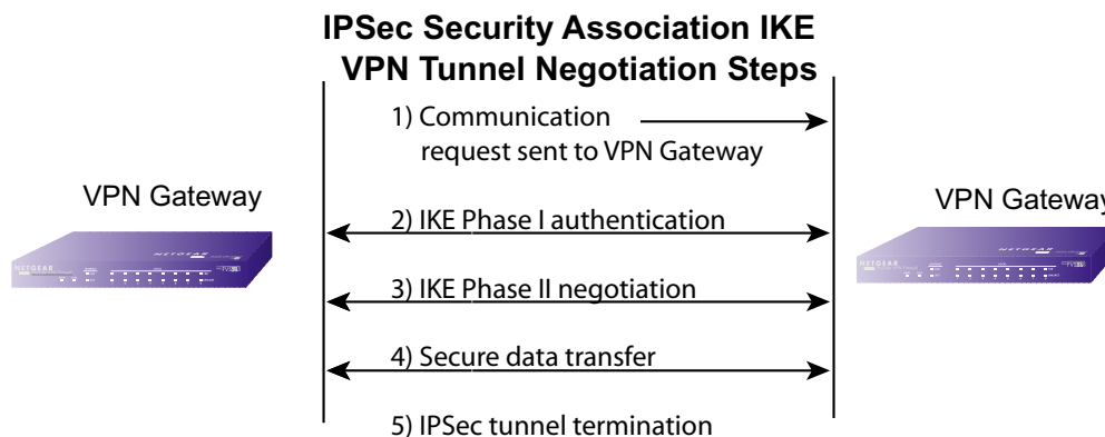
Figure 8-9: IPSec SA negotiation
