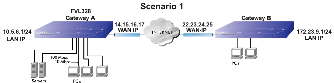
Figure 6-6: LAN to LAN VPN access from an FVL328 to an FVL328
