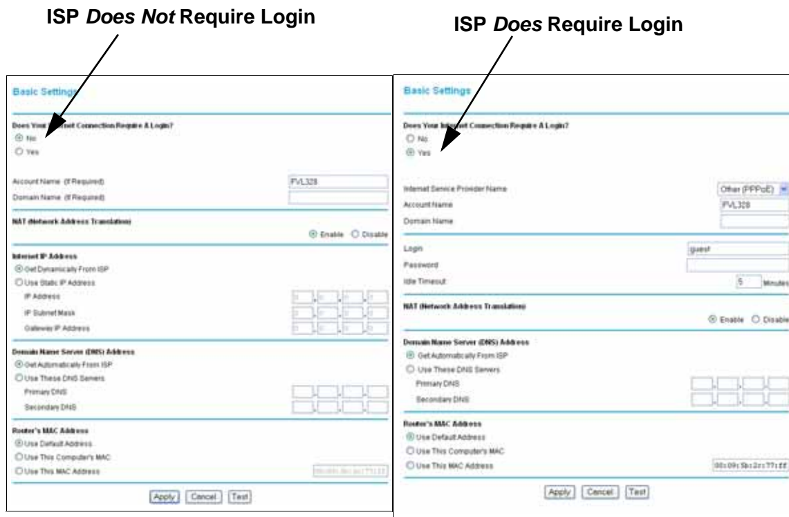
Figure 3-10: Browser-based configuration Basic Settings menu
