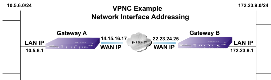
Figure 8-7: VPNC Example Network Interface Addressing
