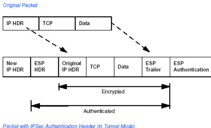
Figure 8-6: Original packet and packet with IPSec ESP in Tunnel mode
