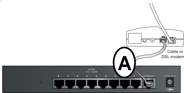
Figure 3-2: Connect the cable or DSL modem to the firewall
