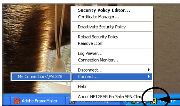
Figure H-13: Connecting the PC to the FVL328 over the VPN tunnel
