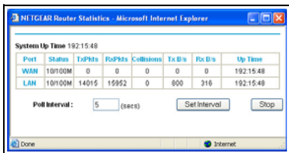
Figure 7-2. Router Statistics screen
