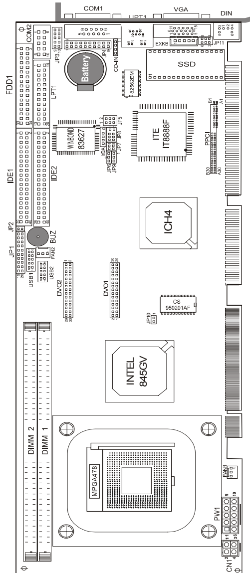
FSC-1716VDN Connector, Jumper and Component locations
