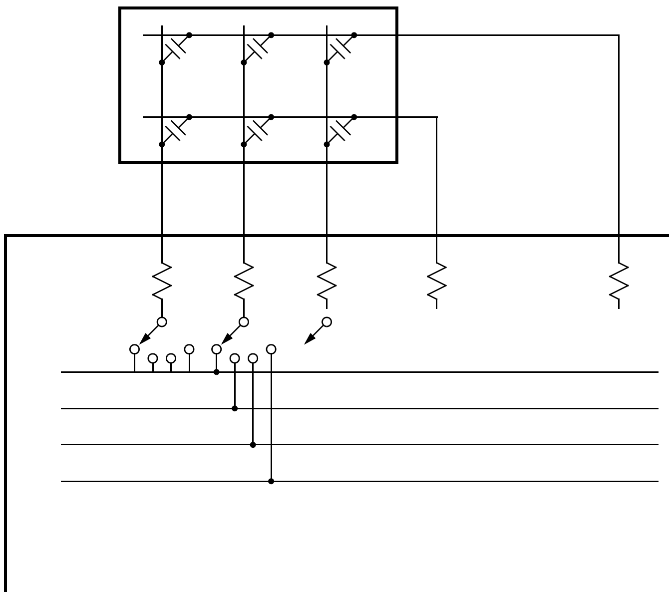
Figure 17-3. Simplified LCD Schematic (1/3 Duty, 1/3 Bias)LCD
