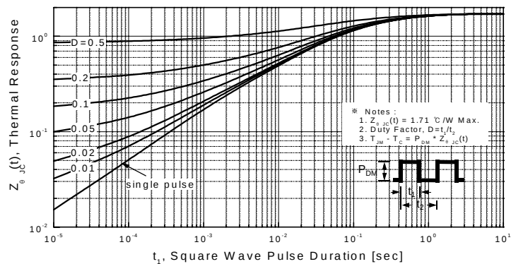
Figure 11-1. Transient Thermal Response Curve for FQP6N40C
