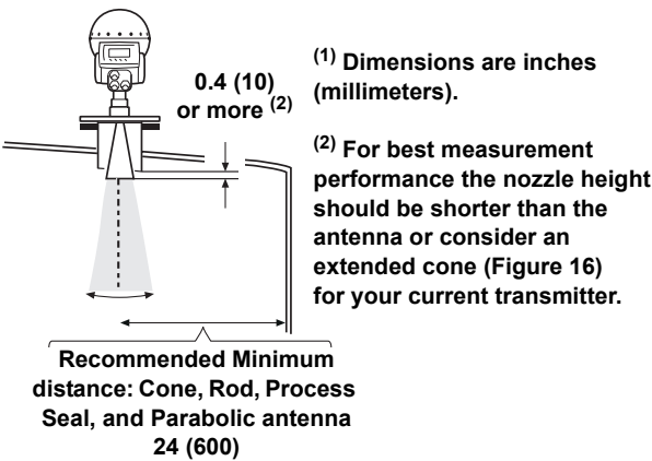
FIGURE 5. Preferred Mounting (1)
