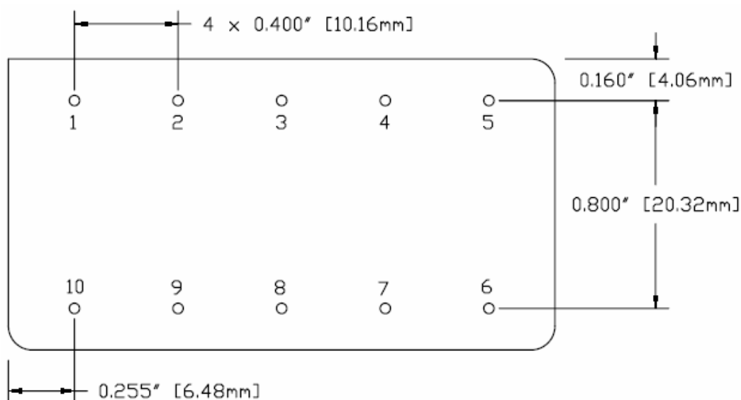
BOTTOM VIEW
