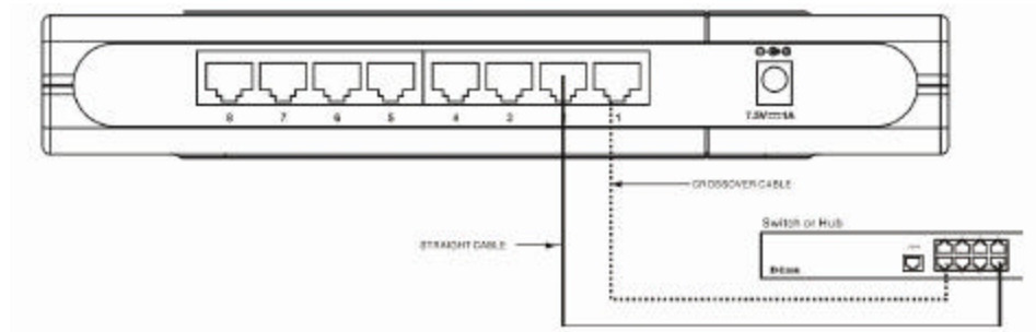
Figure 3-2. Switch connected to a port on a hub or switch using either a straight or crossover cable—any standard Ethernet cable is fine
