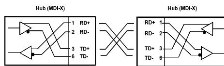
Crossover cable for DES-1008D (MDI-X port) to switch/hub or other network devices (MDI-X port) connection
