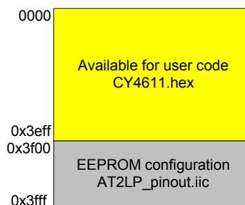
Figure 2: EEPROM memory map
