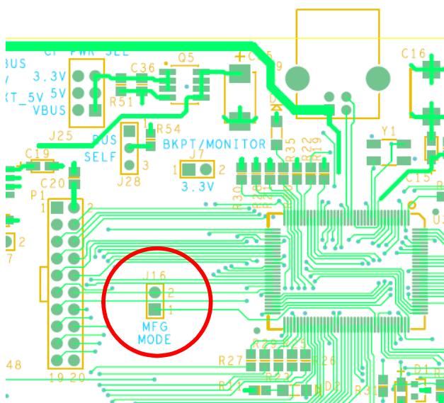
Figure 3: MFG Mode jumper location
