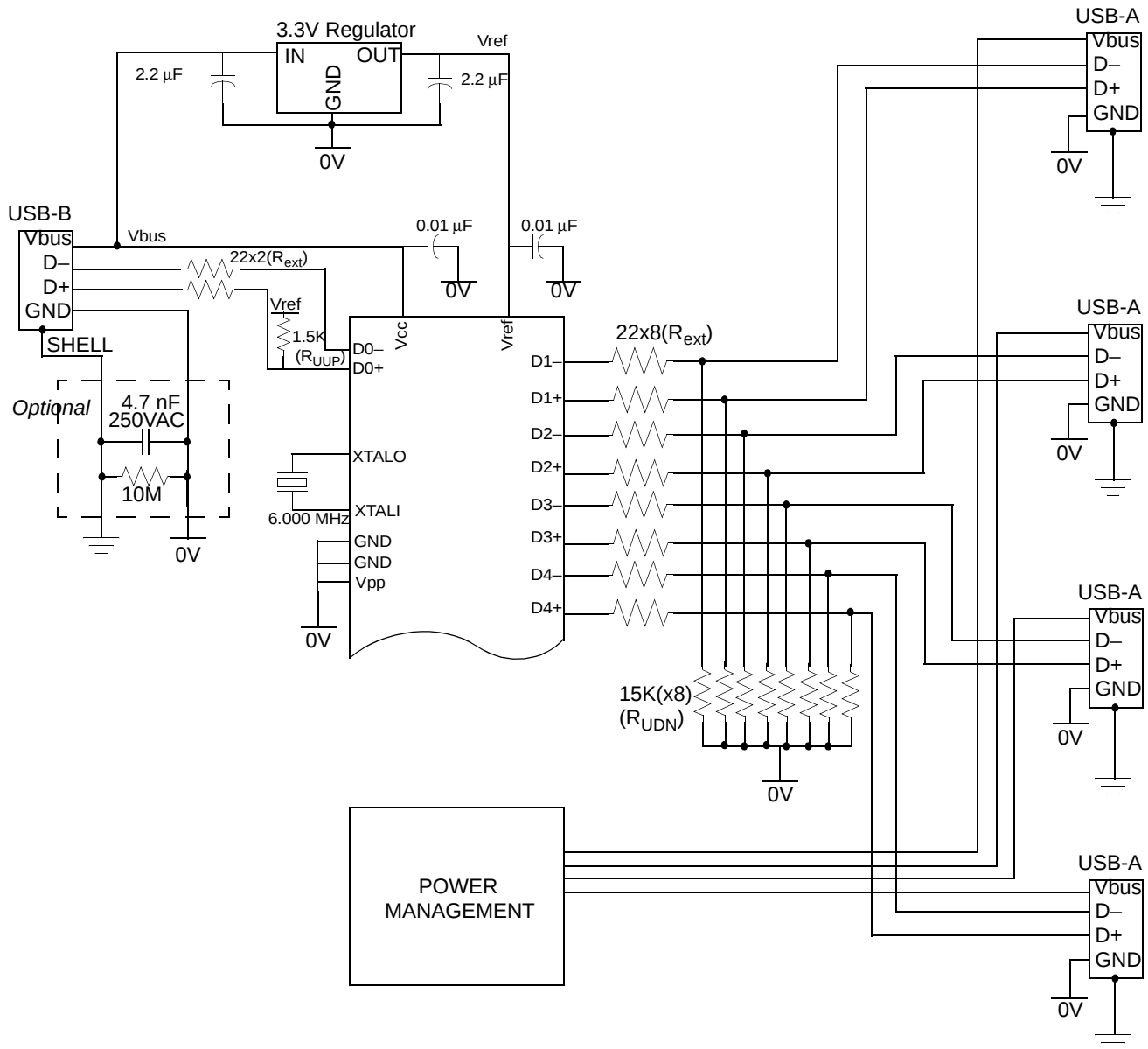
Figure 21-1. Sample Schematic
