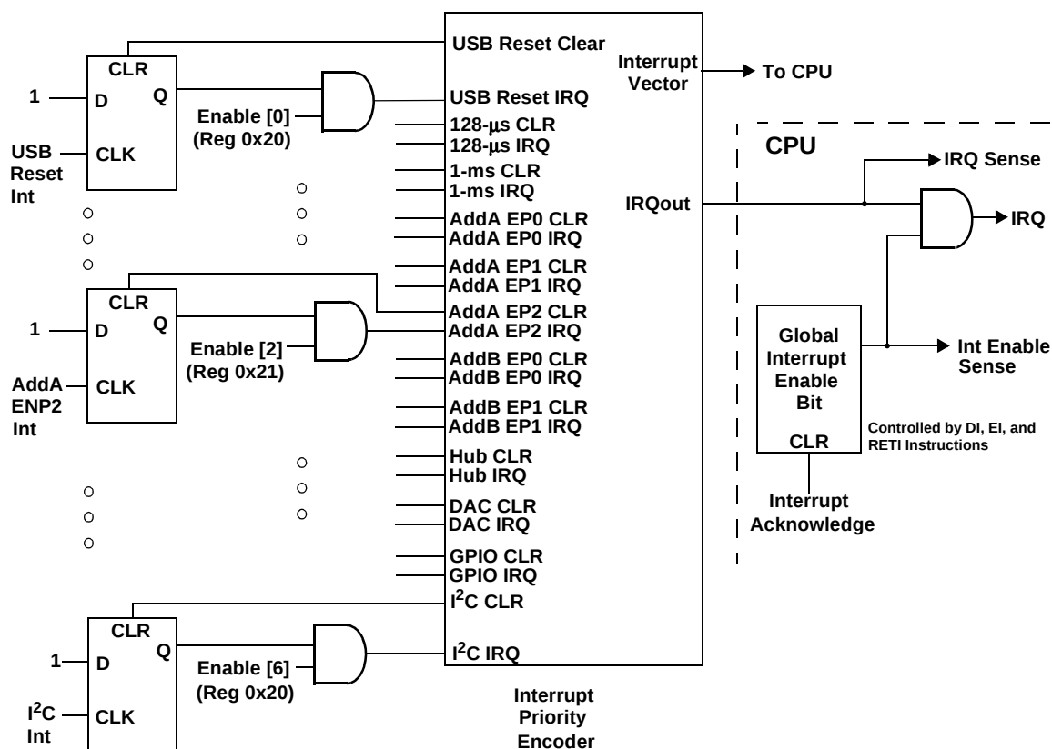
Figure 14-3. Interrupt Controller Functional Diagram
