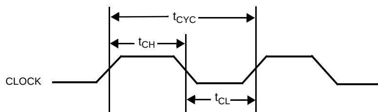
Figure 22-1. Clock Timing
