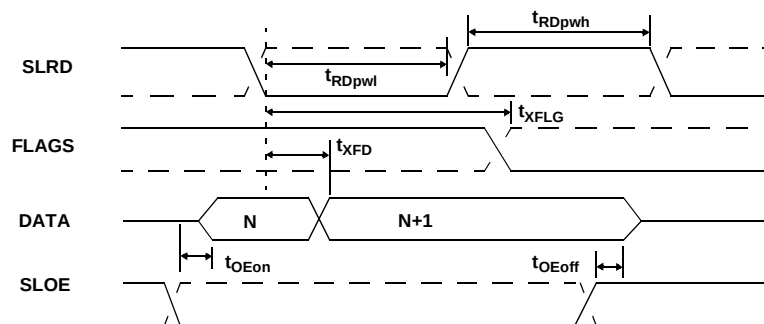
Figure 10-6. Slave FIFO Asynchronous Read Timing Diagram [17]
