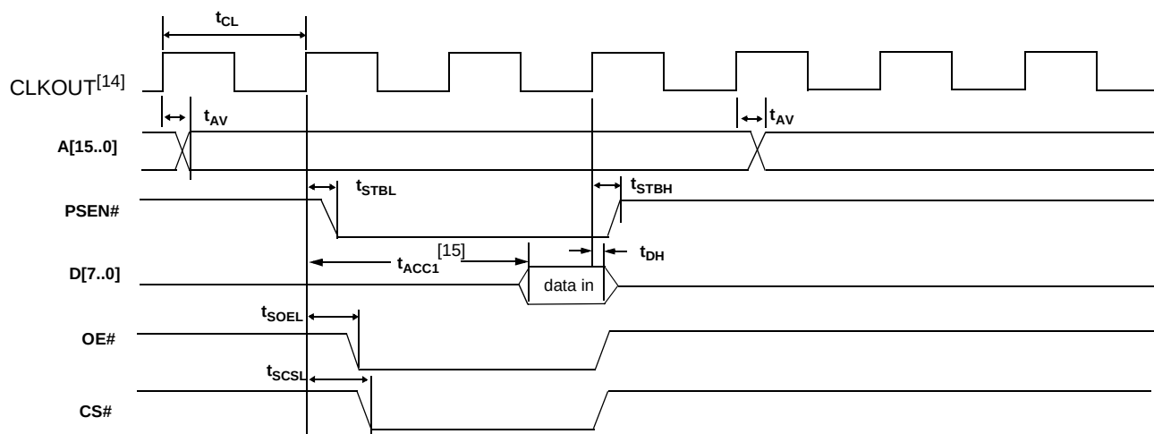
Figure 10-1. Program Memory Read Timing Diagram
