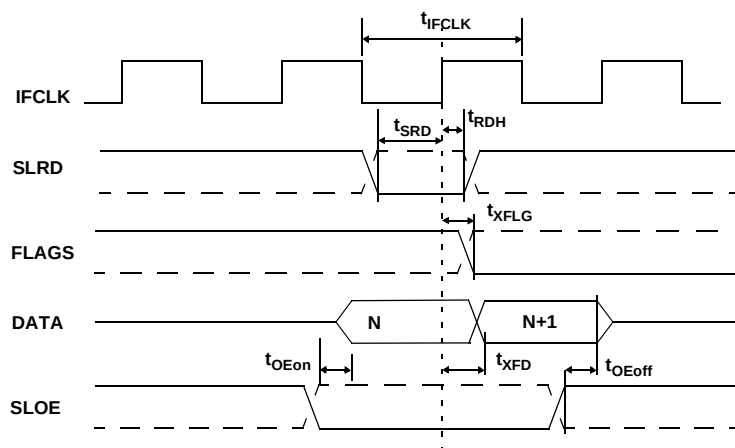
Figure 10-5. Slave FIFO Synchronous Read Timing Diagram [17]
