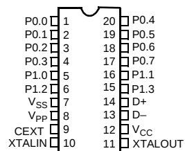
20-pin DIP/SOIC
