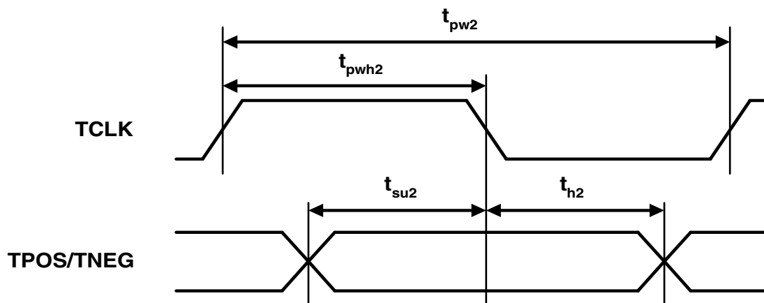
Figure 22. Transmit Clock and Data Switching Characteristics
