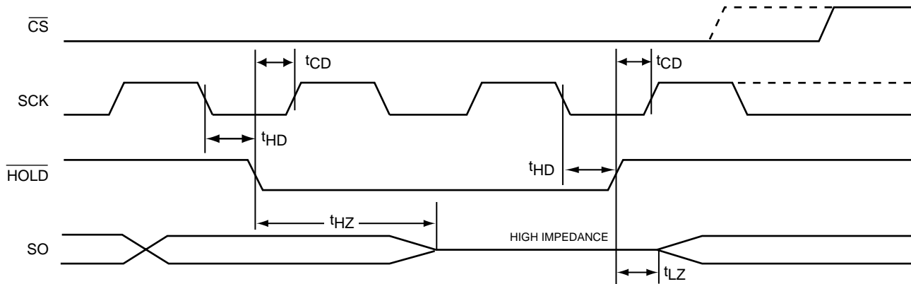
Figure 9. HOLD Timing
