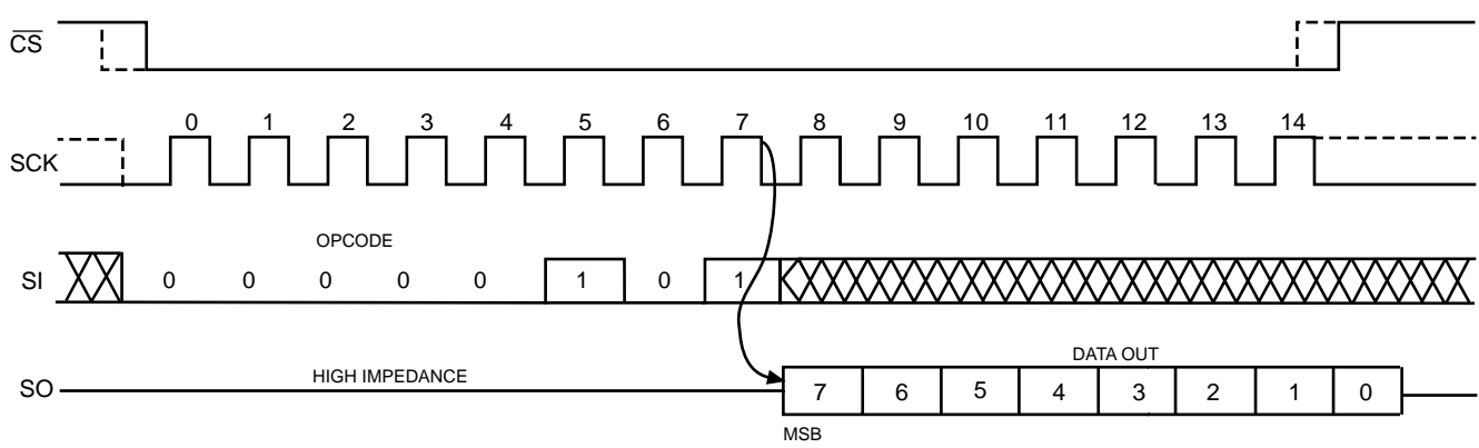
Figure 5. RDSR Timing
