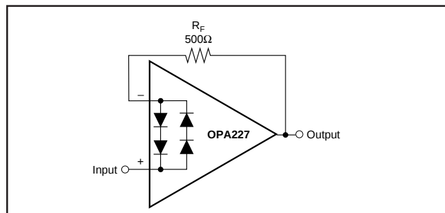
FIGURE 2. Pulsed Operation.
