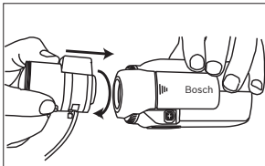
Figure 5.1 Mounting a lens
