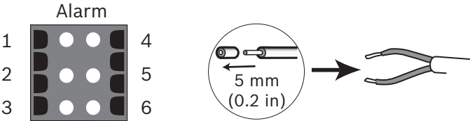
Figure 5.6 Alarm and relay connector pins
