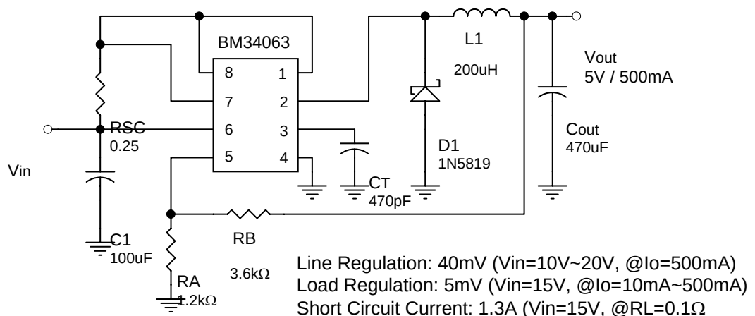
Fig.4 Step-Down Converter
