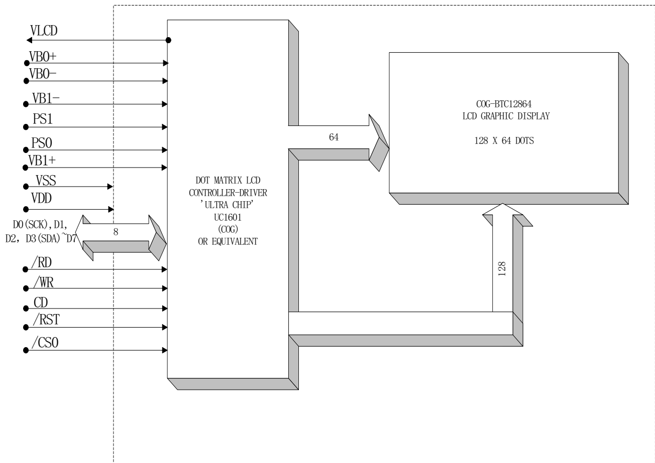
Figure 2: Block diagram
