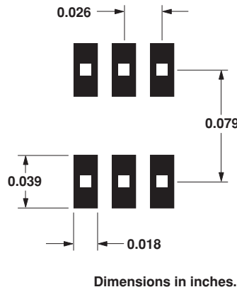
Figure 13. Recommended PCB Pad Layout for Agilent's SC70 6L/SOT-363 Products.
