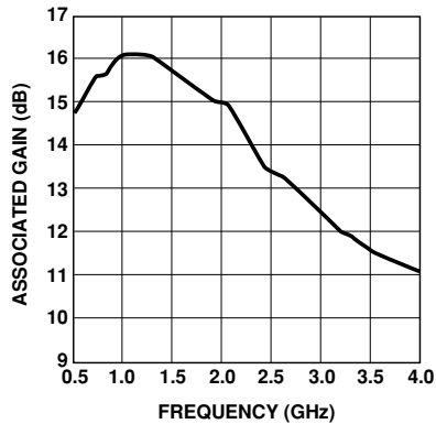
Figure 15. Associated Gain vs. Frequency at V_{dd} = 5 Volts.
