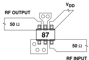
Figure 14. RF Layout.
