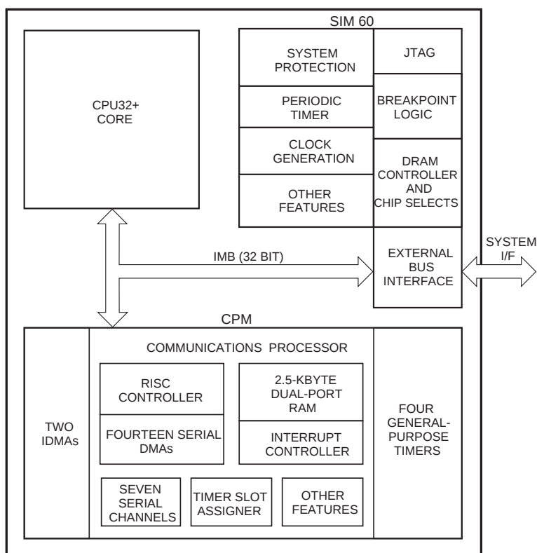
Figure 1. QUICC Block Diagram
