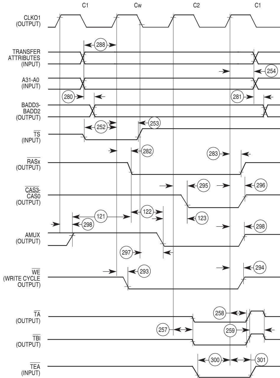
Figure 36. External TS68040 DRAM Cycles Timing Diagram
