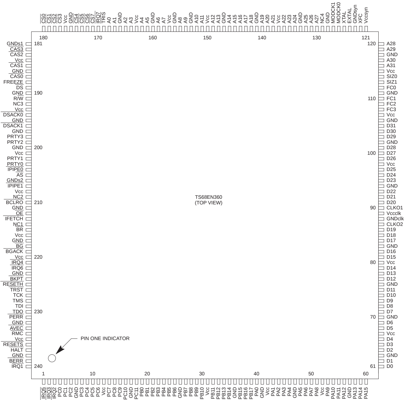
Figure 3. 240-lead Cerquad
