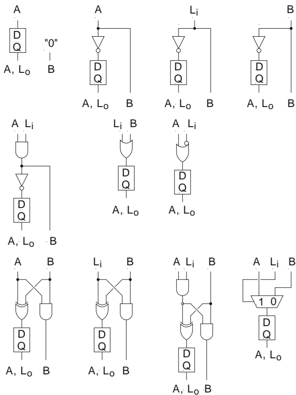
Figure 6. Register States
