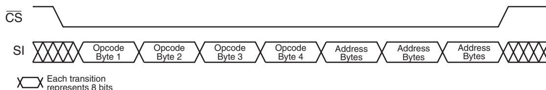
Figure 10-1. Sector Lockdown
