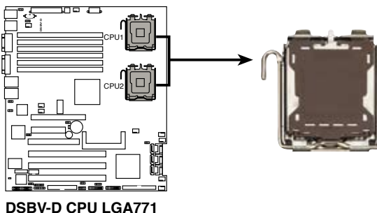
DSBV-D CPU LGA771
